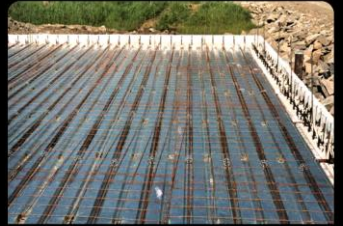
Steel Pan Floor
